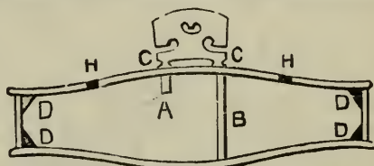
FIG. 83.—Section of the Violin across the f holes.
